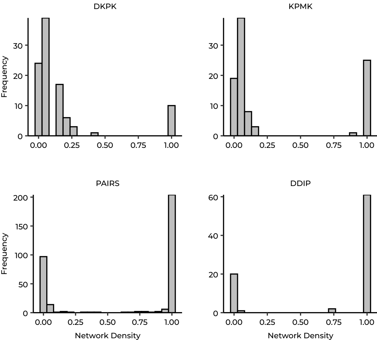
Figure 2 Histograms of the Density of Estimated Temporal Networks for Each Dataset
